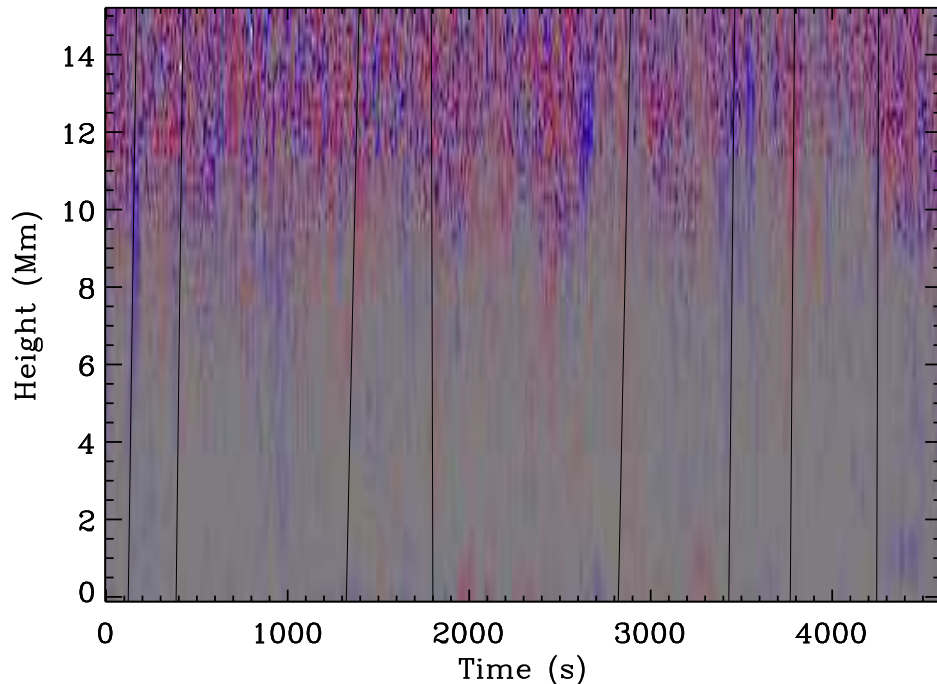
Figure 7. Time-distance plot of \delta\lambda fluctuations, which are proportional to \delta v fluctuations. The color scale is linear from \pm 0.34 \text{ \AA} , with red negative, blue positive, and grey zero. Black lines show the fit to tracked moving structures in the time-distance plot. The slopes of these lines indicate the speed.
