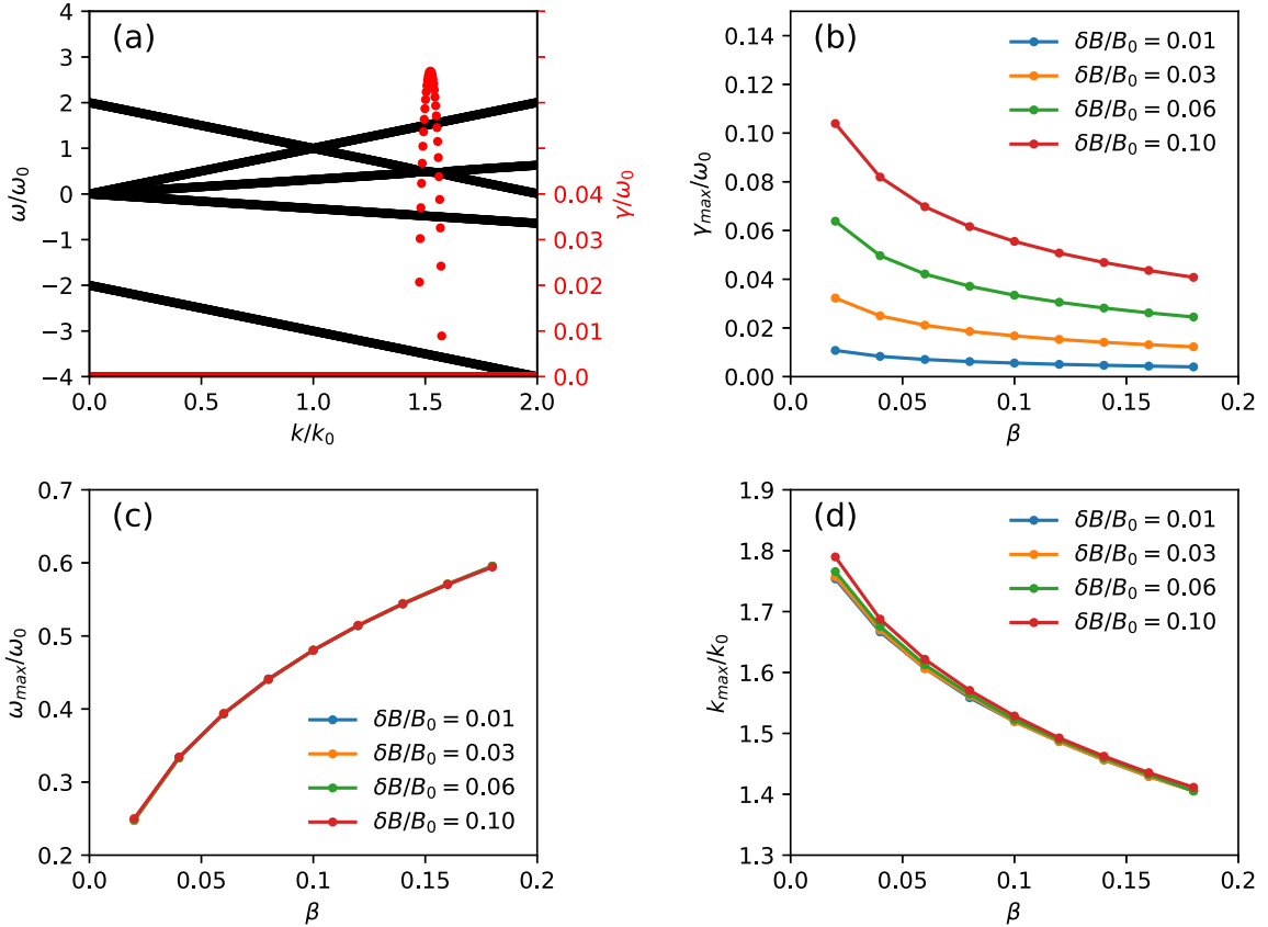
Figure 8. (a) Numerical solutions to the nonlinear dispersion relation for parametric decay instabilities of an Alfvén wave (Derby, Jr. 1978) with \delta B/B_0 = 0.06 and \beta = 0.1 . The black dots, which blend together to appear as black lines, show real frequencies \omega , and the red dots show growth rates \gamma , both of which are normalized to the frequency of the pump Alfvén wave \omega_0 . The wavenumbers are normalized to the wavenumber of the pump wave k_0 (note that \omega_0 = k_0 V_A ). At any given k there are five solutions, most of which are stable (i.e. \gamma = 0 ). The unstable solution near k/k_0 = 1.53 corresponds to PDI, with a maximum growth rate \sim 0.032 , and frequency \sim 0.48 . (b) The growth rate, (c) the frequency, and (d) the wavenumber of the most unstable (largest \gamma ) PDI mode for various combinations of \delta B/B_0 and \beta . All three quantities depend on \beta , but \omega_{max} and k_{max} have little dependence on \delta B/B_0 (In (c) four curves lie on top of one another).
