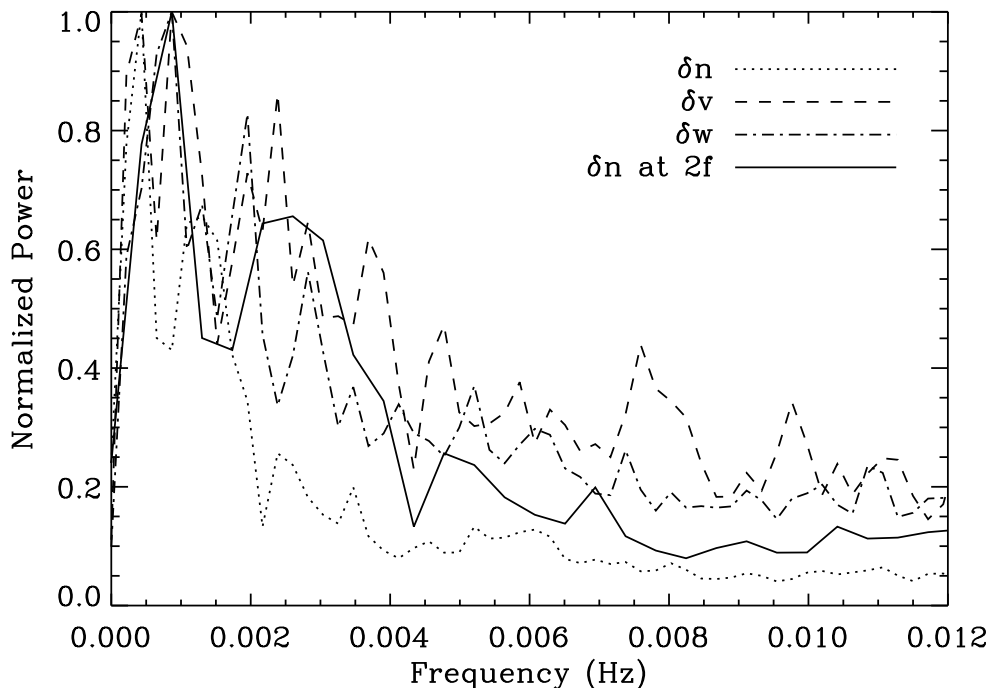
Figure 4. Average power spectrum for the density fluctuations (labeled \delta n ; dotted curve), velocity fluctuations (labeled \delta v ; dashed curve), and line width fluctuations (labeled \delta w ; dash-dotted curve), normalized to their respective maximum values. The solid curve shows the average power spectrum for the density fluctuations when its frequency axis is multiplied by a factor of two. In that case, the peaks \delta n power spectrum align better with peaks in the \delta v and \delta w power spectra. The relative uncertainties in the normalized power are estimated to be about 13%.
