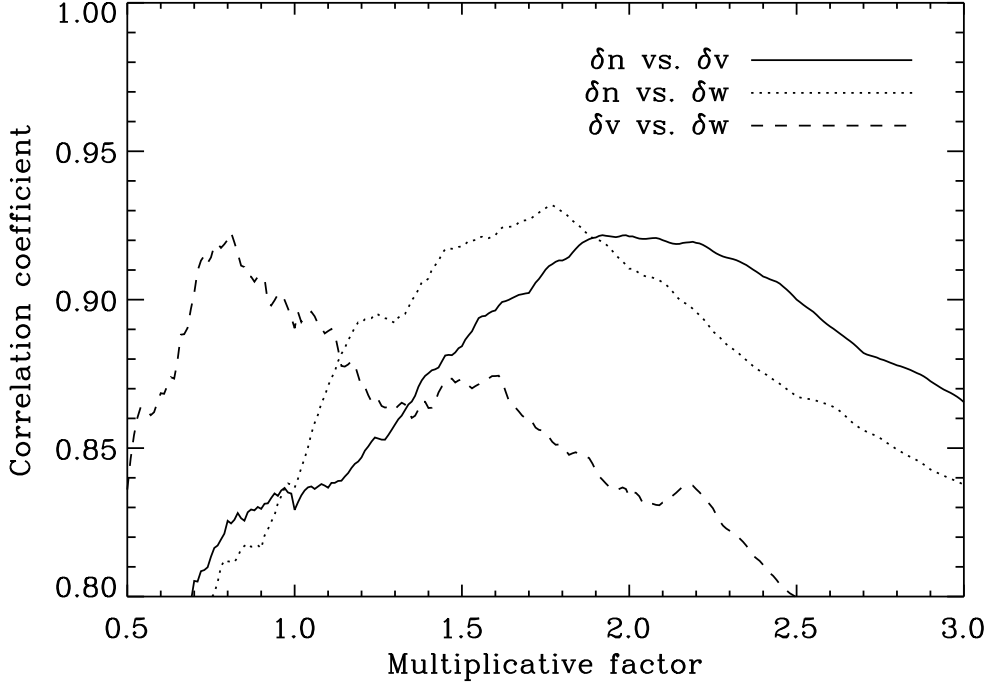
Figure 5. Correlation coefficient versus the scaling factor for the frequency axis for the power spectra of \delta n vs. \delta v (solid curve), \delta n vs. \delta w (dotted curve), and \delta v vs. \delta w (dashed curve). In each case, it is the first variable listed whose frequency axis is to be multiplied.
