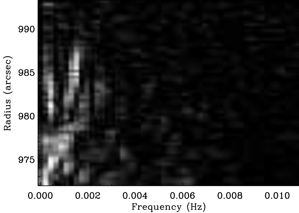
Figure 2. Power spectrum of the relative density fluctuations as a function of height. Here the power spectrum is normalized by the total power at each height. The color scale is linear with a maximum value of 0.15 shown in white and zero in black.
